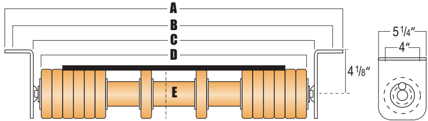
Series 25 – 5 inch Spool Type Roller
